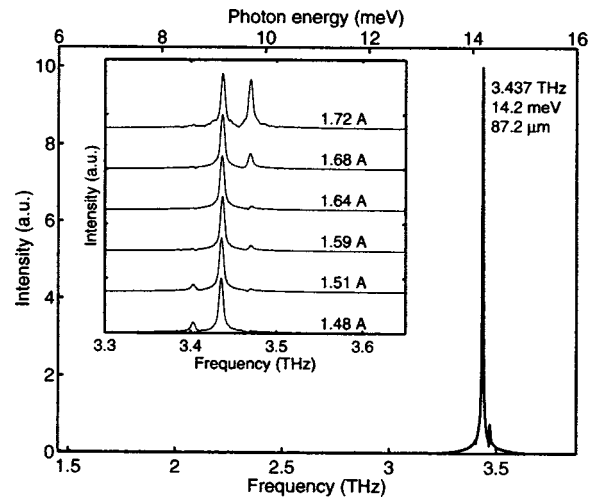
FIG. 2. Emission spectrum above threshold biased at 1.64 A with 100-ns pulses repeated at 10 kHz, at T = 5 \text{ K} . Spectra were measured with a Ge:Ga photodetector from Infrared Labs. The inset shows an expanded view of spectra at various bias points, offset for clarity. The spectra were collected using a Nicolet 850 Fourier transform spectrometer in linear-scan mode, and the measured linewidth is limited by the instrumental resolution of 3.75 GHz.
