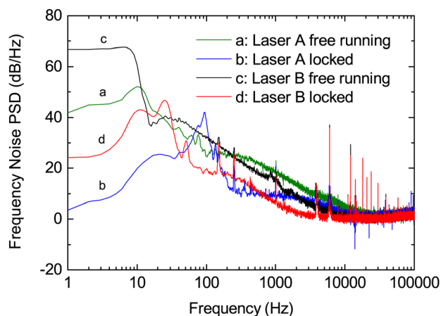
FIG. 4. (Color online) Frequency noise power spectral density of the lock-in signal for two lasers in the free running and locked states.
