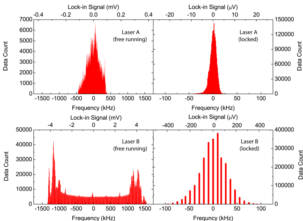
FIG. 3. (Color online) Histogram of the relative frequency deviation to the center frequency for two lasers in the free running and locked states, calculated based on the lock-in signal fluctuations of a 10 s observation time.
