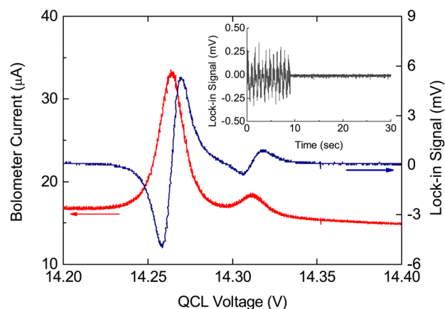
FIG. 2. (Color online) Absorption profile of methanol lines at 1.1 mbar as measured for “laser A.” By using a NbN bolometer detector and a lock-in amplifier, the error signal was measured, labeled as lock-in signal. The voltage window (linear region for the lock-in signal) used for lock-in feedback loop is 8 mV. The inset shows the lock-in signal in the unlocked and locked state after about 8 s for “laser A.”
