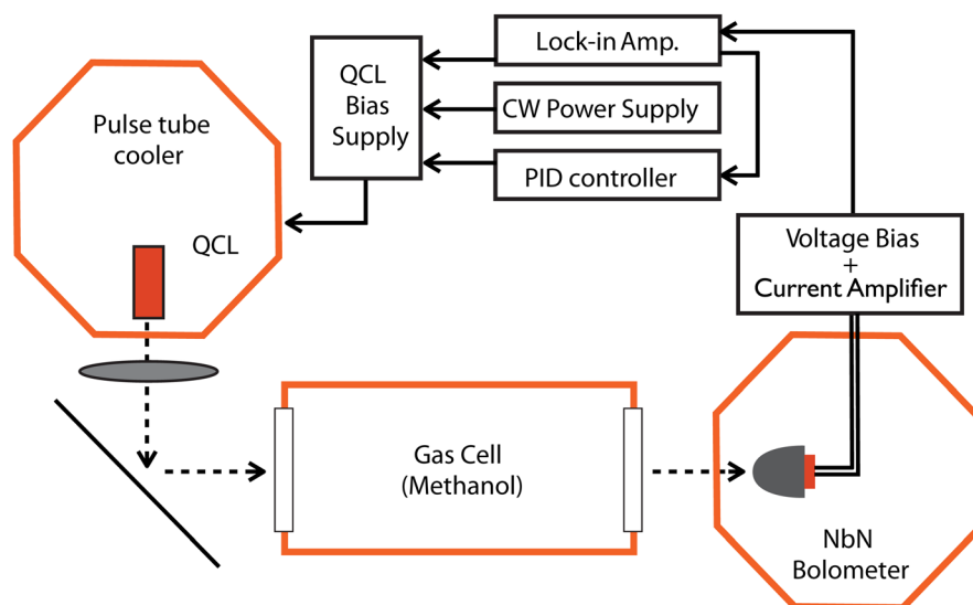
FIG. 1. (Color online) Schematic of the frequency locking measurement setup.
